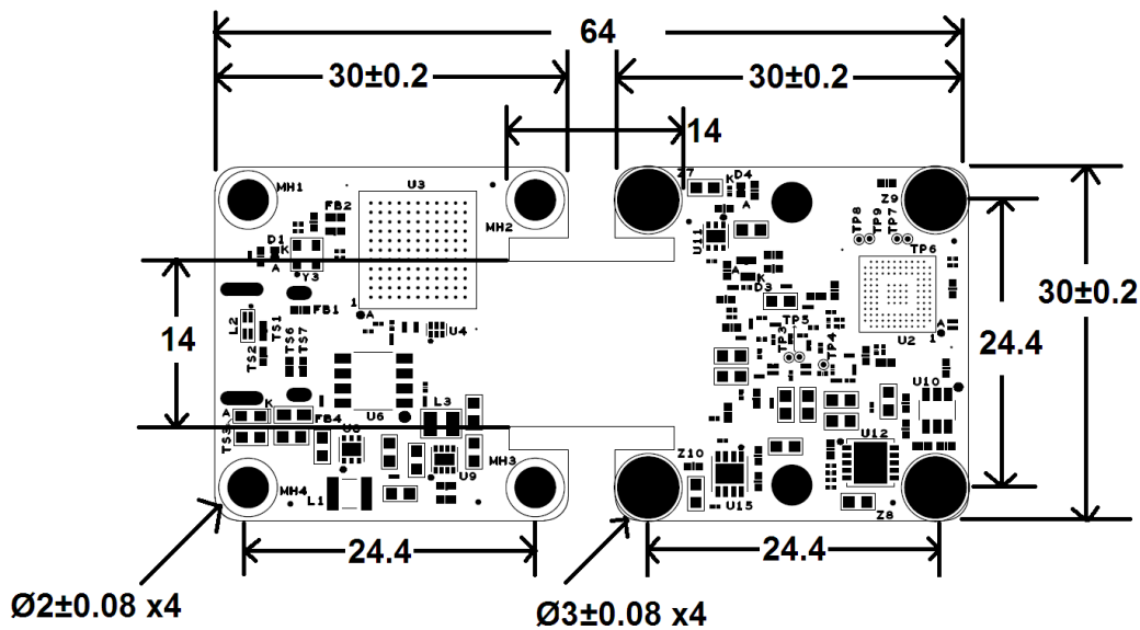
Figure 5: Top View of See3CAM_24CUG_CH_TC Mechanical Dimensions
