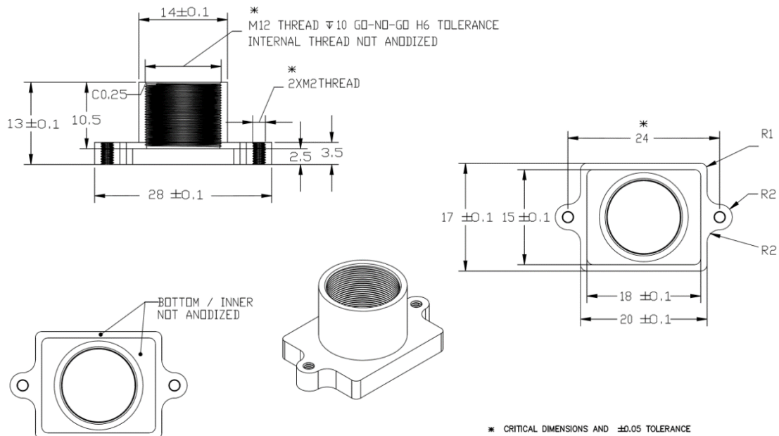
Figure 8: Lens Holder Mechanical Dimensions
