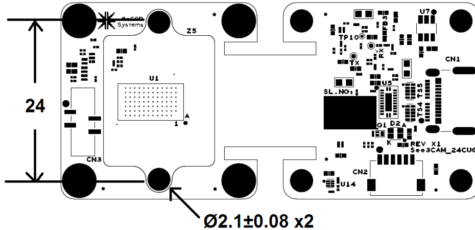
Figure 6: Bottom View of See3CAM_24CUG_CH_TC Mechanical Dimensions
