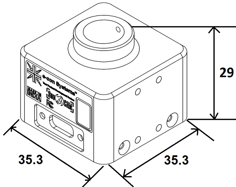
Figure 7: See3CAM_20CUG_CH_TC_BX Dimensions (Without lens)
