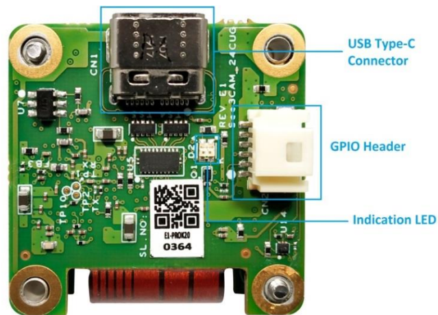
Figure 4: GPIO Header of See3CAM_24CUG_CH_TC
